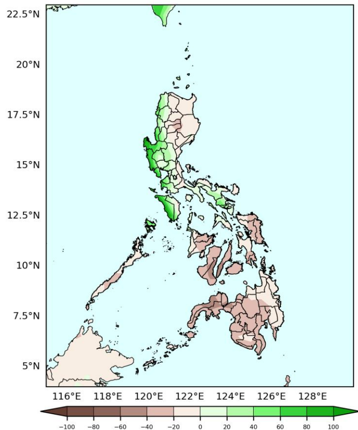
GEFS Week-2 Precip Anomaly
